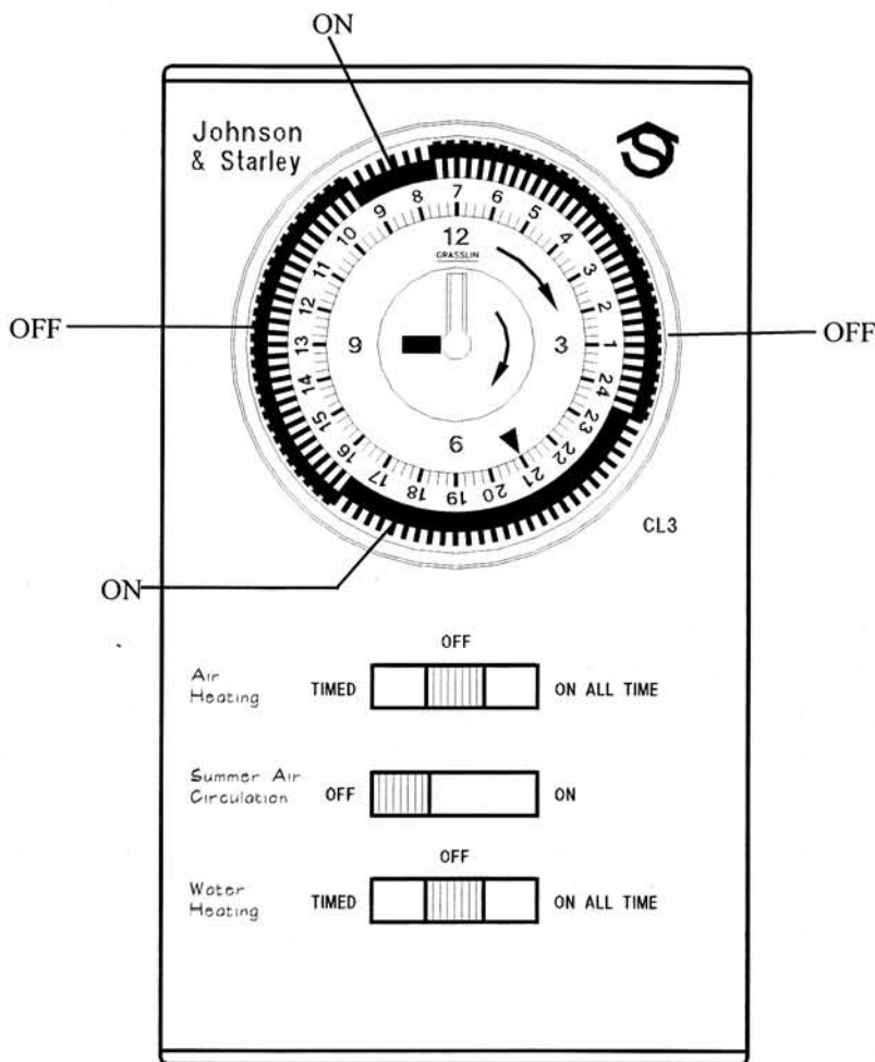
Fig. 2 Integral Time Control
